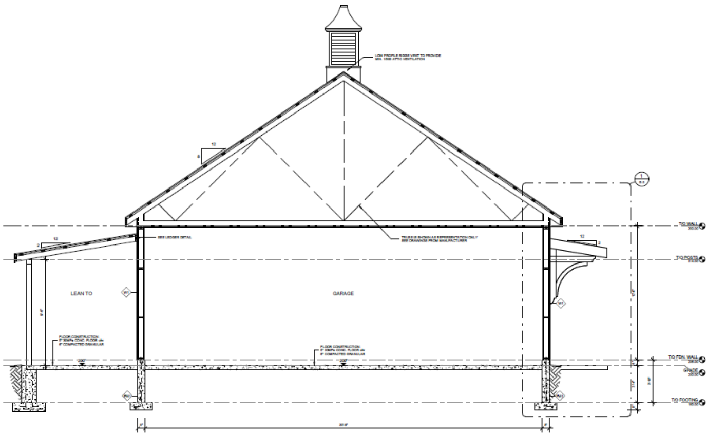
1 BUILDING SECTION S-2 3/8" = 1'-0"
