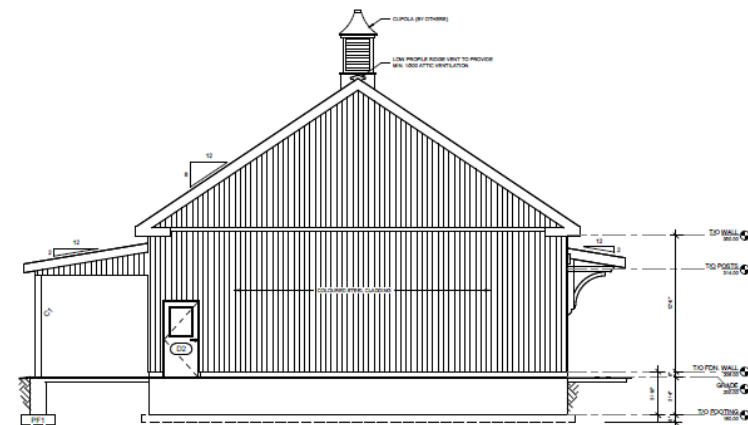
2 PROJECT WEST ELEVATION S-4 1/8" = 1'-0"
