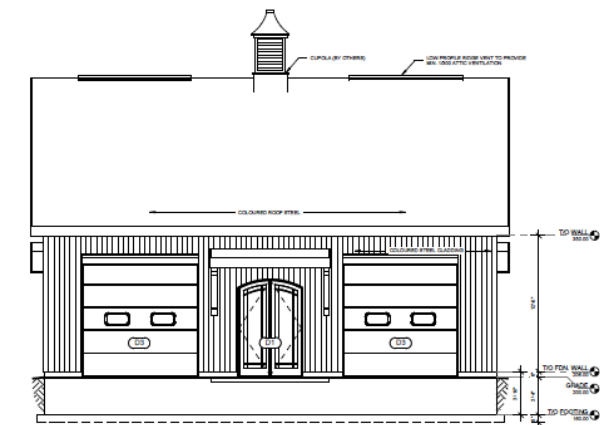
1 PROJECT SOUTH ELEVATION S-4 1/8" = 1'-0"
